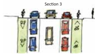
40 Foot Road = 6' 1' 7' 12' 7' 1' 6'
