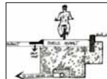
Porous, Raised Bike Lane
